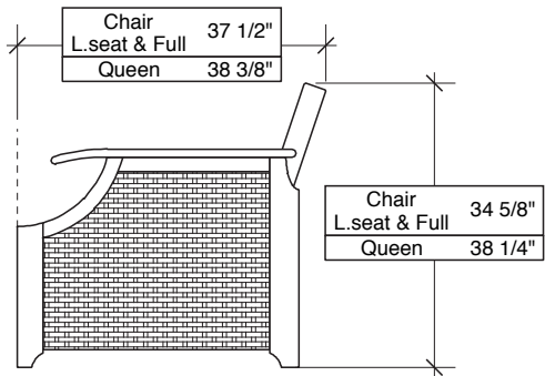
SEATING POSITION
